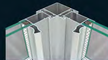
Corner Standard Connection
