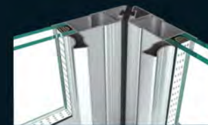
Corner 45 degree Connection
